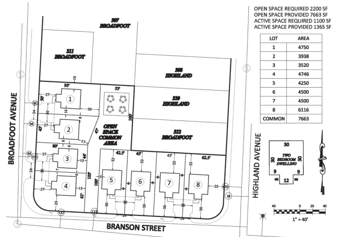
Friendship House Cottage Site Plan
