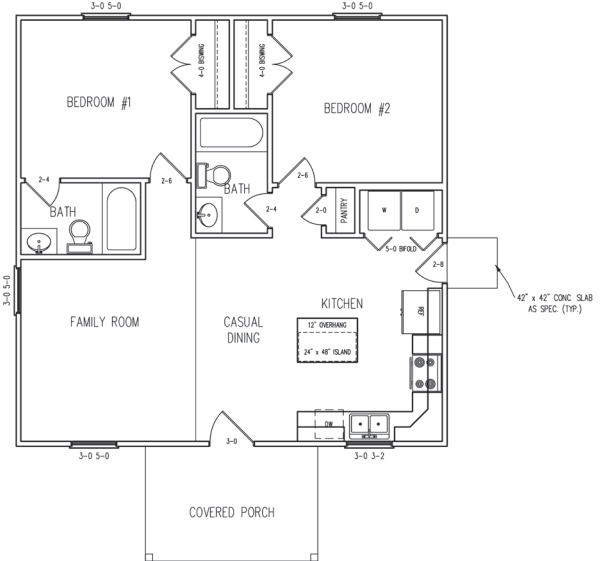
Friendship House Cottage Floor Plan
